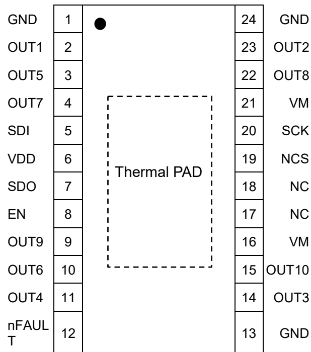
Figure 2. NSD8310 Pinout
