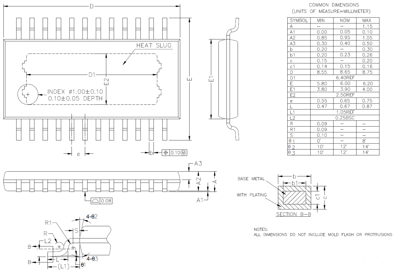
Figure 15. NSD8310A package information
