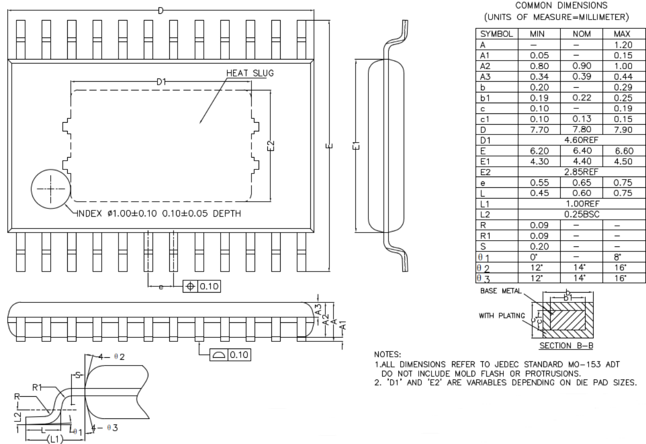
Figure 14. NSD8310 package information
